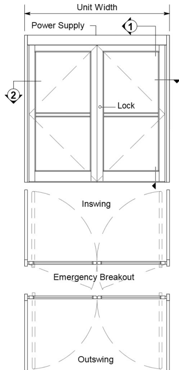
Exterior Elevation and Floor Plan
