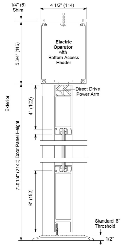
Vertical Section '1'
